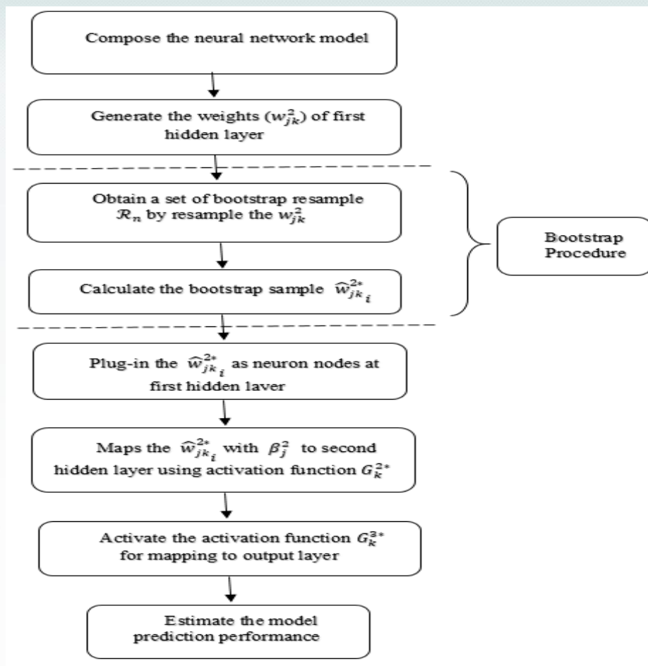
Figure 2. Bootstrapping The Hidden Layer of Neural Network Prediction Model.
