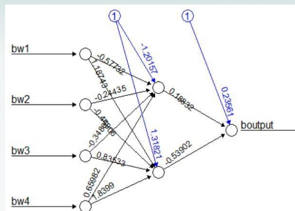
Figure 6. Bootstrap the weight of first hidden layer neural network
