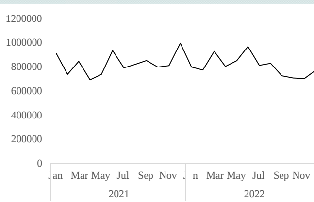
Figure 7. Predicting the Singaporean guest visiting Malaysia during COVID-19 crisis.
